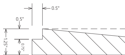
Low Profile Offset Drain Pan
